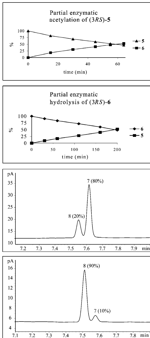
Figure 1. Kinetics of enzymatically catalysed acetylation of (3 RS )- 5 and enzymatically catalysed hydrolysis of (3 RS )- 6 ; GLC analysis of compounds 7 and 8 produced by spiroketalization of 5 after enzymatic acetylation and enzymatic hydrolysis, respectively
