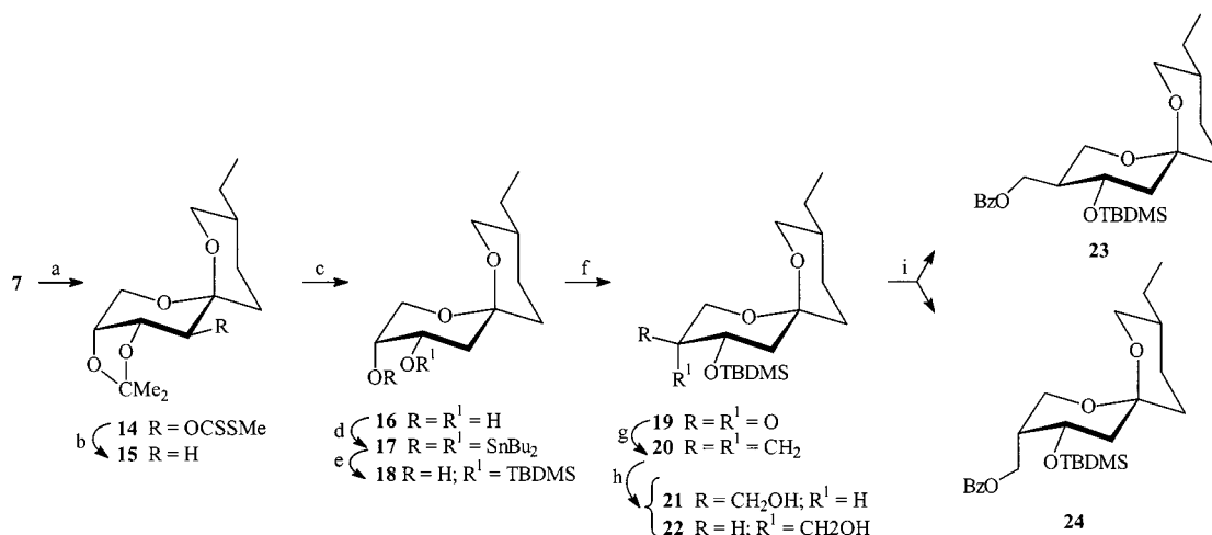
Scheme 6. Synthesis of protected (–)-talaromycins B ( 23 ) and A ( 24 ): a: NaH/THF/imidazole/ \text{CS}_2 /MeI; b: \text{H}_3\text{PO}_4 /dioxane/ \text{H}_2\text{O} / \text{Et}_3\text{N} /AIBN; c: AcOH/ \text{H}_2\text{O} /50 °C/1 h; d: n\text{Bu}_2\text{SnO} /MeOH; e: TBDMSCl/dioxane; f: PCC/ \text{CH}_2\text{Cl}_2 /NaAcO/MS (4 Å); g: \text{NaCH}_2\text{SOCH}_3 / \text{Ph}_3\text{PCH}_3\text{Br} /DMSO; h: \text{BH}_3 - \text{SMe}_2 /THF, then NaOH/ \text{H}_2\text{O}_2 ; i: BzCl/ \text{Et}_3\text{N} / \text{CH}_2\text{Cl}_2
