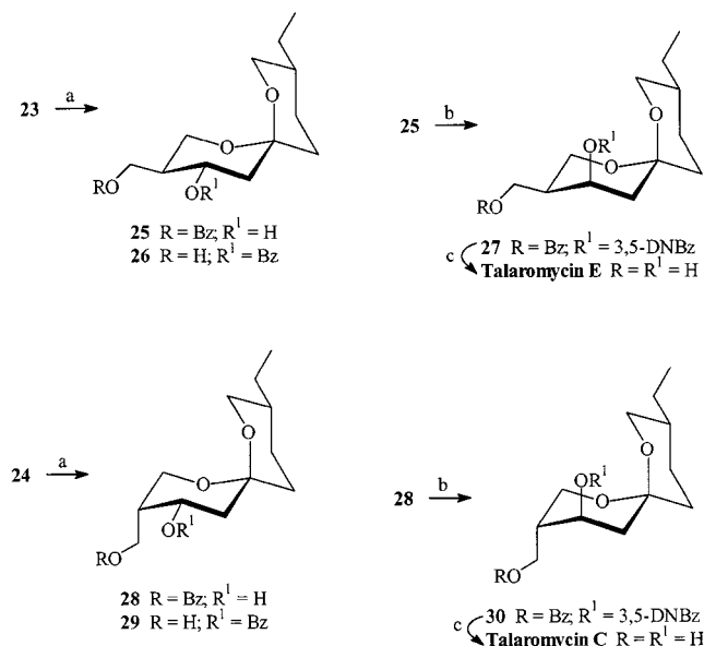
Scheme 7. Synthesis of (–)-talaromycins E and C: a: n\text{Bu}_4\text{NF}\cdot 3\text{H}_2\text{O}/\text{THF} ; b: \text{Ph}_3\text{P}/3,5\text{-dinitrobenzoic acid}/\text{DEAD}/48\text{ h}/\text{room temp.} ; c: \text{NaMeO}/\text{MeOH}
